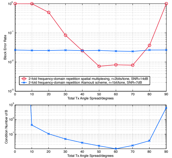
Fig. 1. Impact of total transmit angle spread on performance of space-frequency codes.
